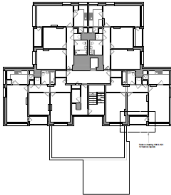
TYPICAL FLOOR
