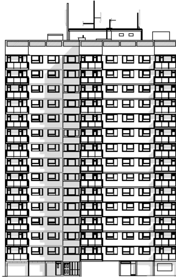
WEST ELEVATION
